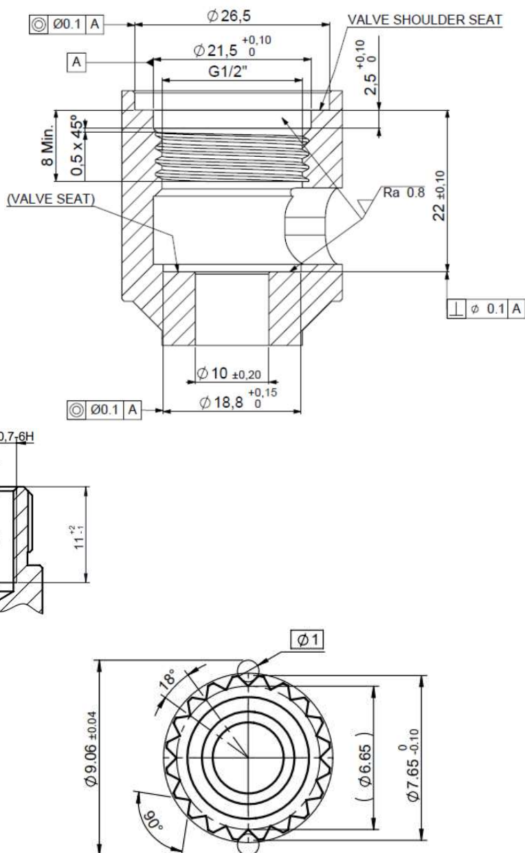
DETAIL D Teeth Z=20
