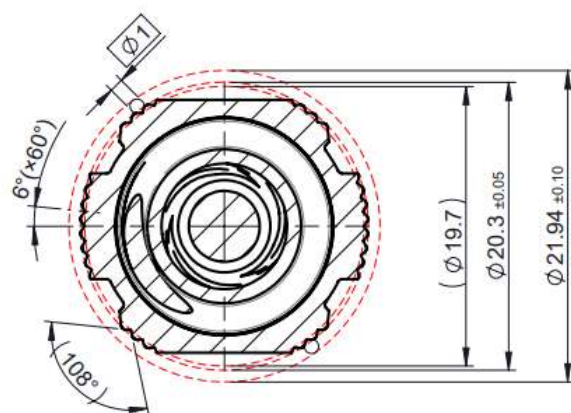
SECTION O-O SCALE 2 : 1 60 Teeth
