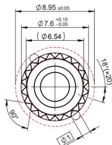
SHAFT Milling detail SCALE 4 : 1 20 Teeth
